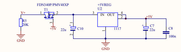
+5V SELECTOR (USB)
